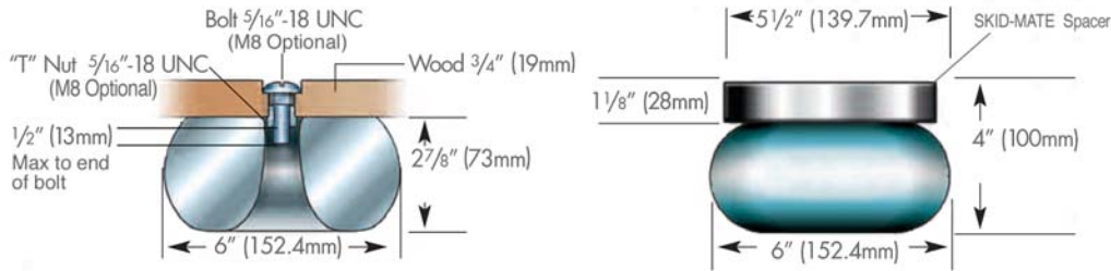
Typical SKID-MATE pallet for heavy and sensitive loads.
